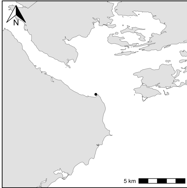
Figure 2: Location of ADCP deployed at the Eddy Cove NE station in Strait of Canso in 2014.
