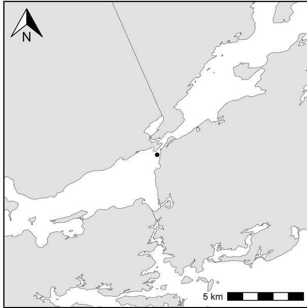
Figure 2: Location of ADCP deployed at the Little Narrows S station in Whycomomagh Bay in 2023.
