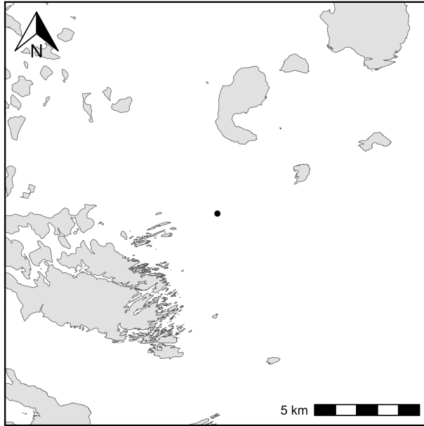
Figure 2: Location of ADCP deployed at the Heckmans Island station in Mahone Bay in 2022.
