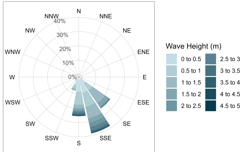
Figure 6: Wave height and the direction the wave is travelling from (relative to True North).
